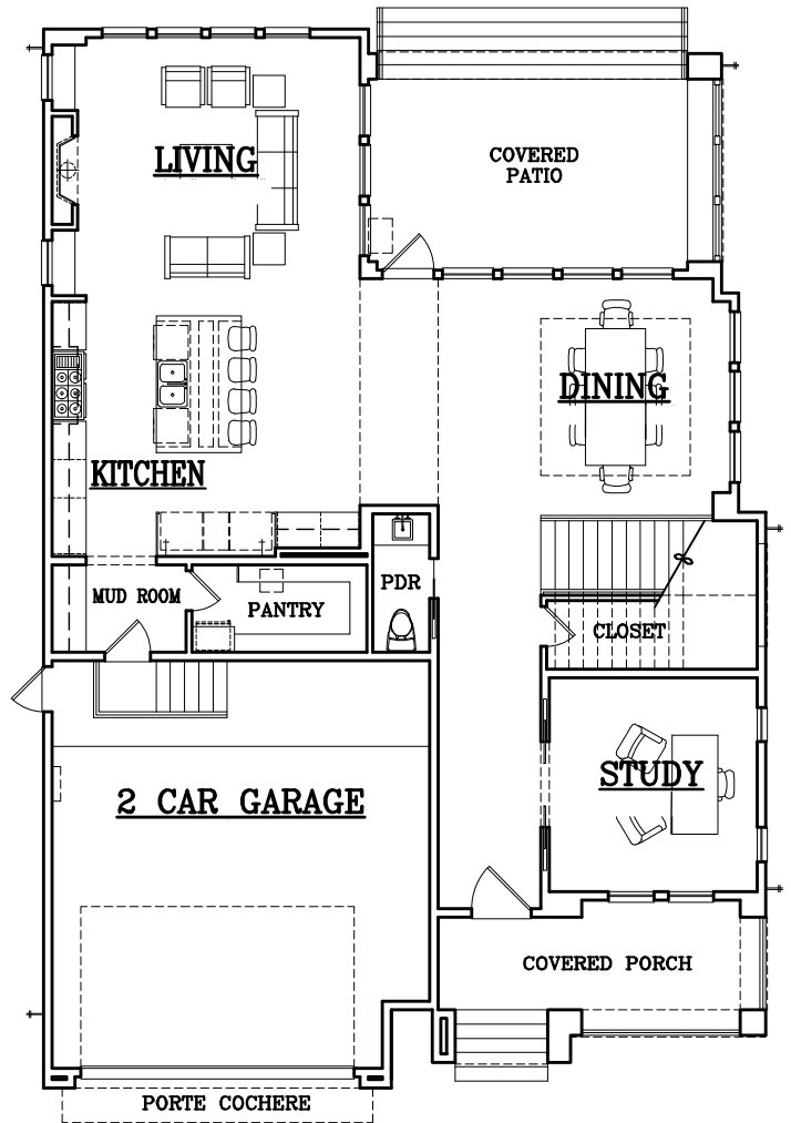
FIRST FLOOR
